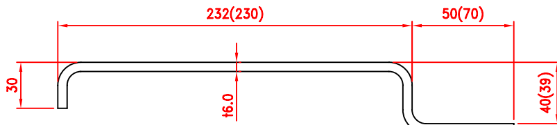
Rear Corner Post Outer
