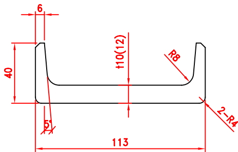
Rear Corner Post Inner
