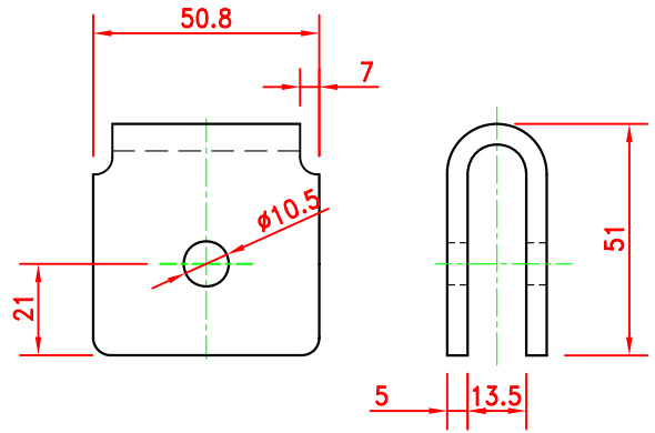
L&R-D23-11 Handle Hub
