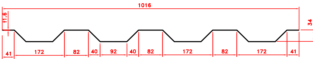
HANJIN Side Panel
