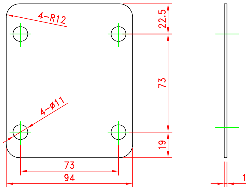
Large Bracket Gasket L&R-DGE06
