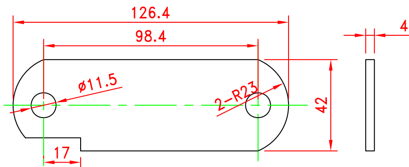
Retainer Bracket Gasket L&R-DGE08040 (4MM )
