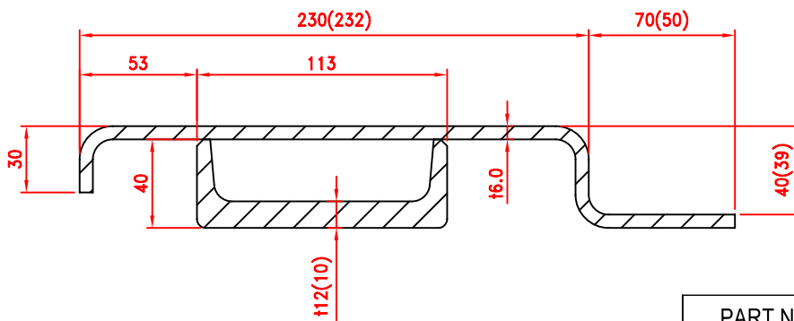
Rear Corner Post
